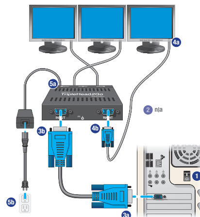
Matrox TripleHead2Go Analog Edition
