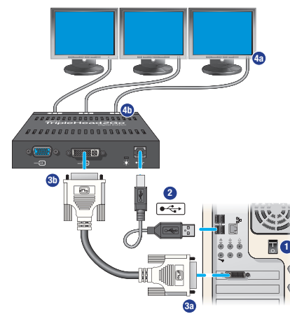
Matrox TripleHead2Go Digital Edition
