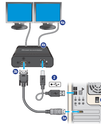
Matrox DualHead2Go DP Edition
