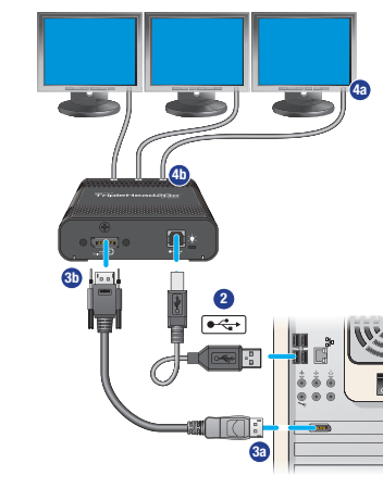
Matrox TripleHead2Go DP Edition
