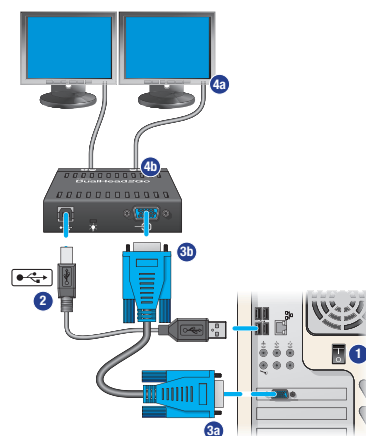
Matrox DualHead2Go Analog Edition
